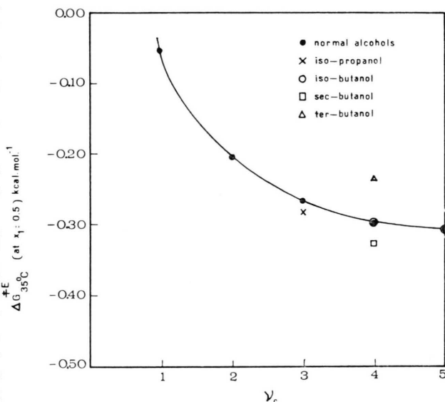
Fig. 3. Variation of the excess free energy of activation ( \Delta G^\ddagger E ) with the number of carbon atoms in alcohols ( \nu_c ) at 35^\circ °C and x_1 = 0.5 .
